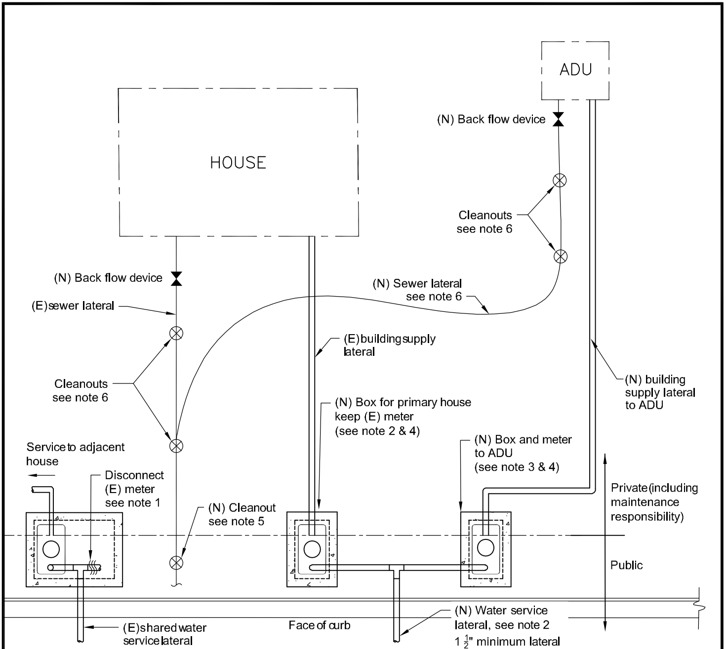
FIGURE 1 PLAN VIEW
