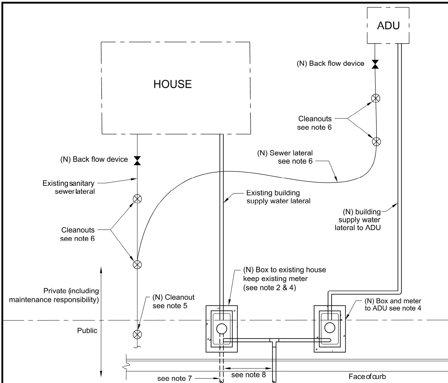
PLAN VIEW
